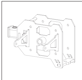
Position 16 1× Pulley Trolley
