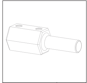
Position 21 1× Cable Termination
