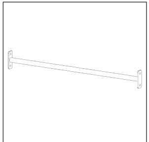
Position 33 | 2×
